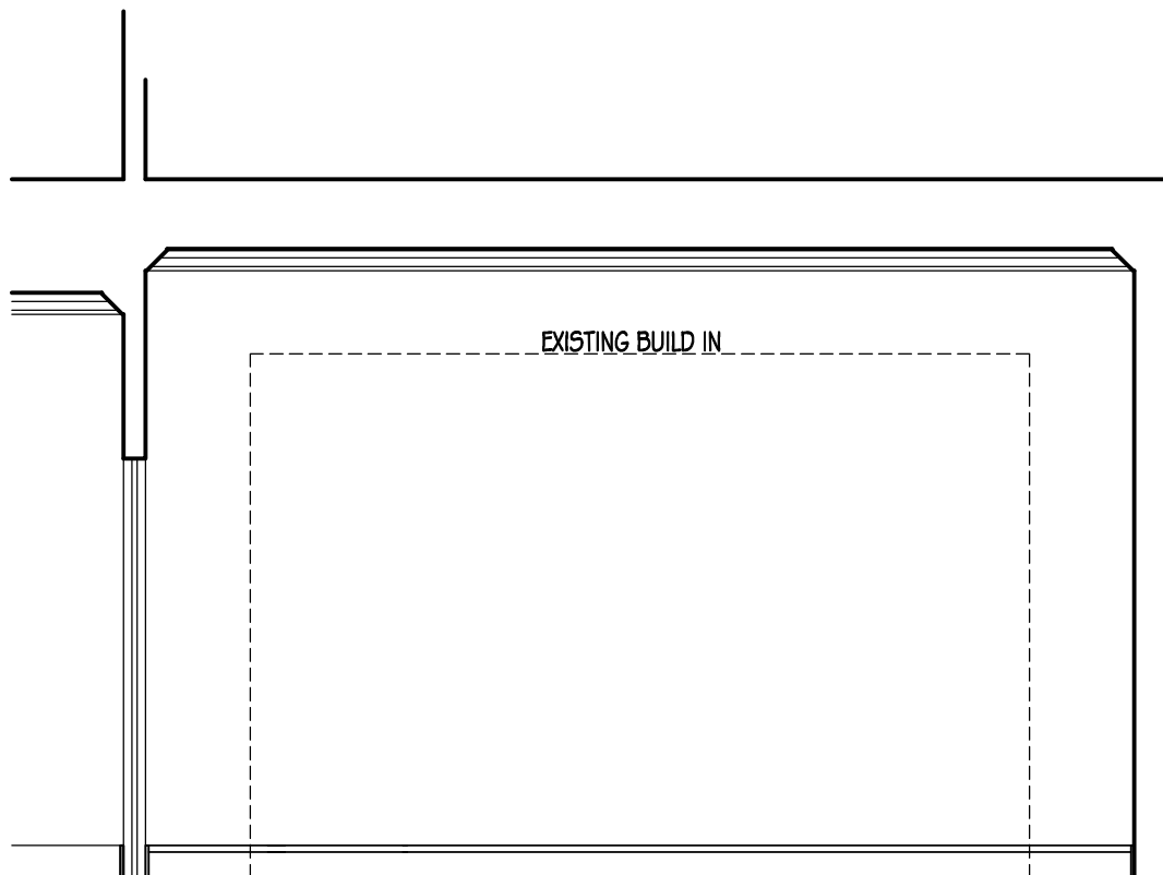
08 - GREAT ROOM SCALE: 1/4" = 1'-0"
