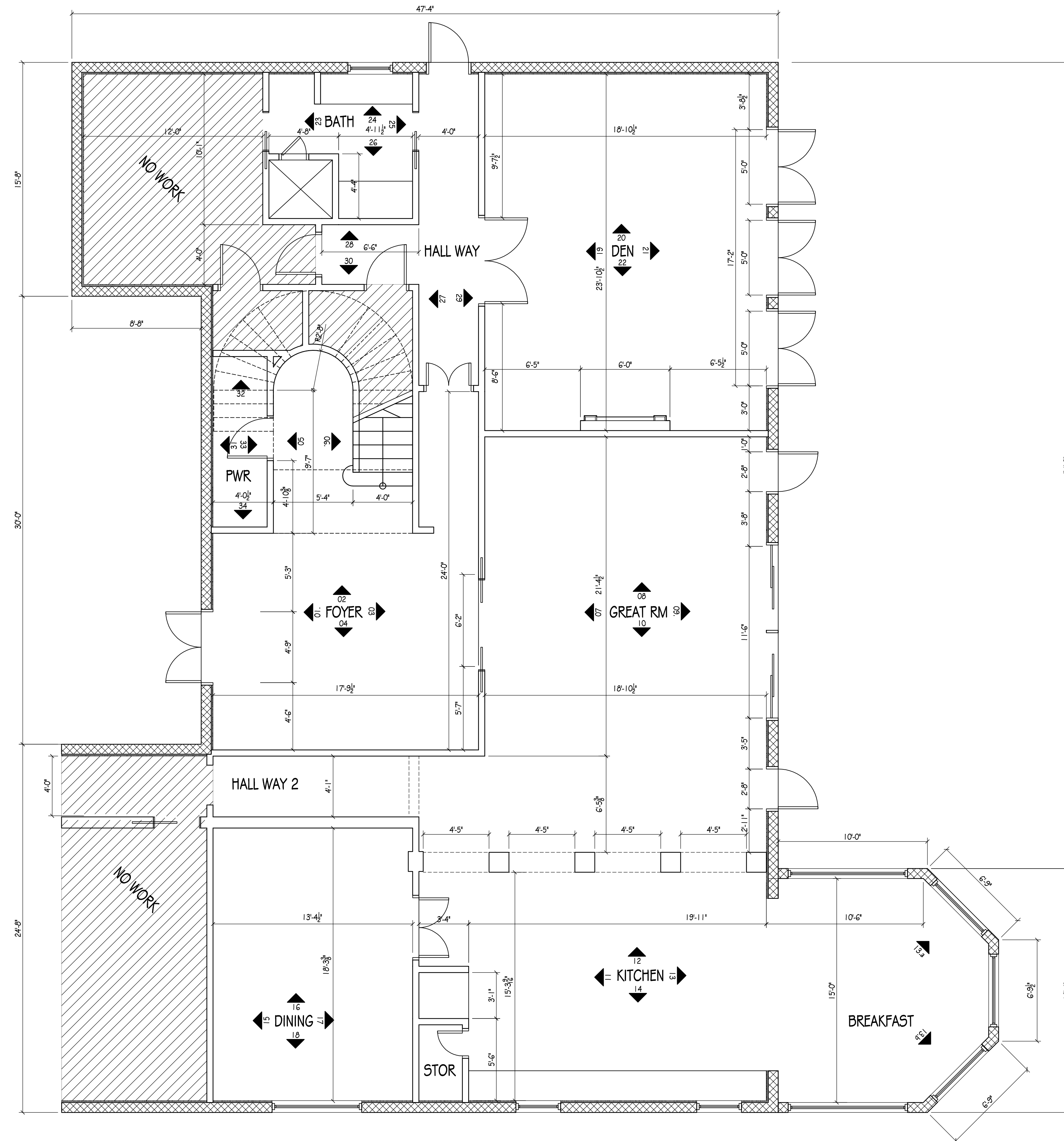
FIRST FLOOR - FLOOR PLAN 1/4" = 1'-0"
