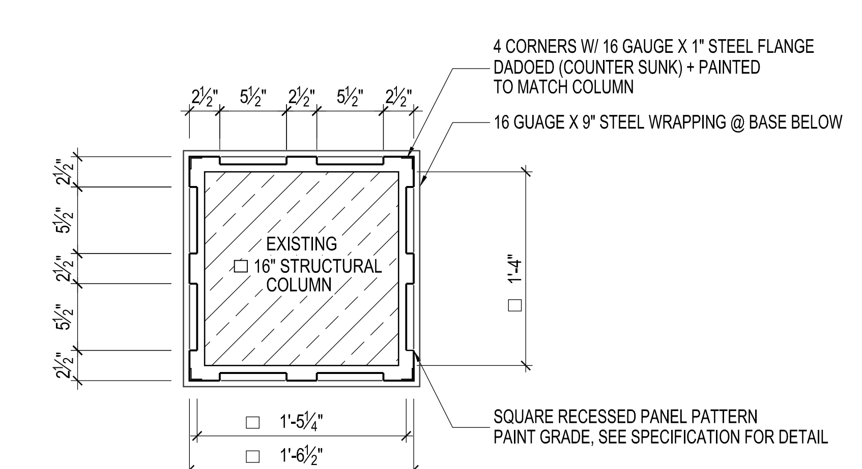
6 PLAN VIEW WOOD COLUMN CLADDING (REF SHEET I0.01) SCALE: 1-1/2" = 1'-0"
