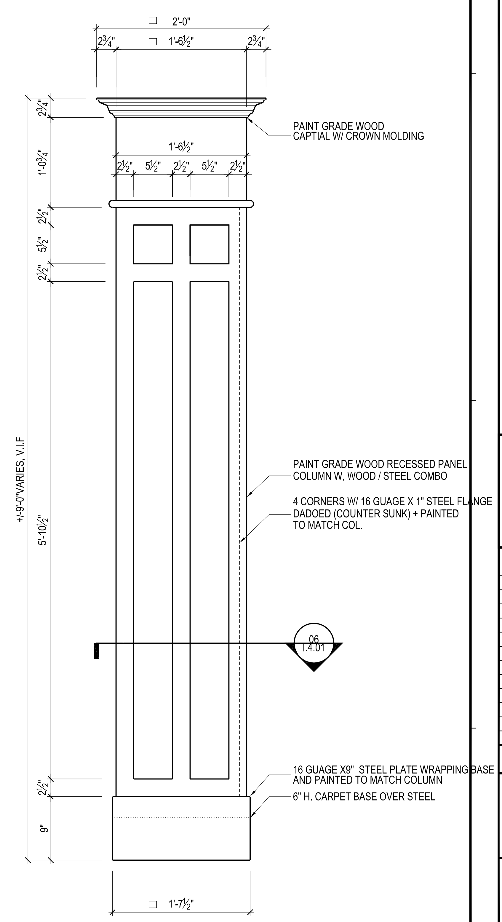
4 ELEVATION WOOD COLUMN CLADDING SCALE: 1-1/2" = 1'-0"
