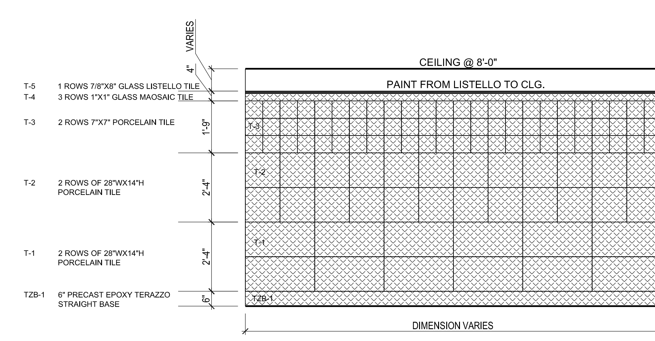
2 ELEVATION BATHROOM WALLS - TYPICAL DETAIL SCALE: 1/2" = 1'-0"
