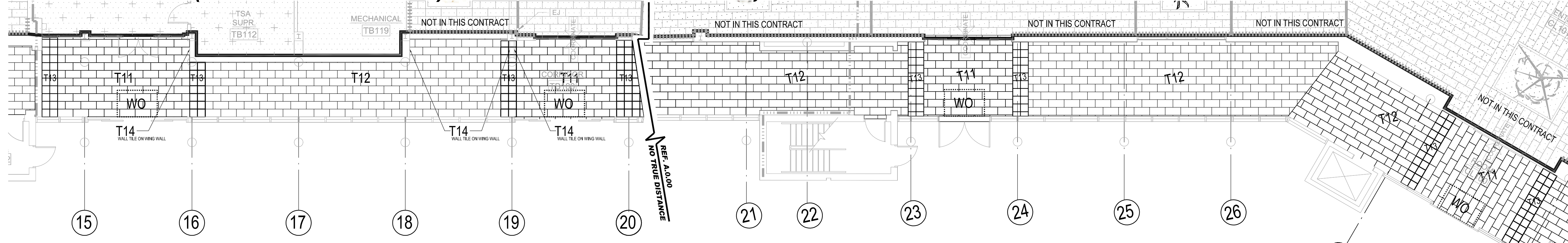
PERIMETER WALKWAY (OUTSIDE TICKETING B) FLOOR PLAN, SCALE: 1/8" = 1'-0"
