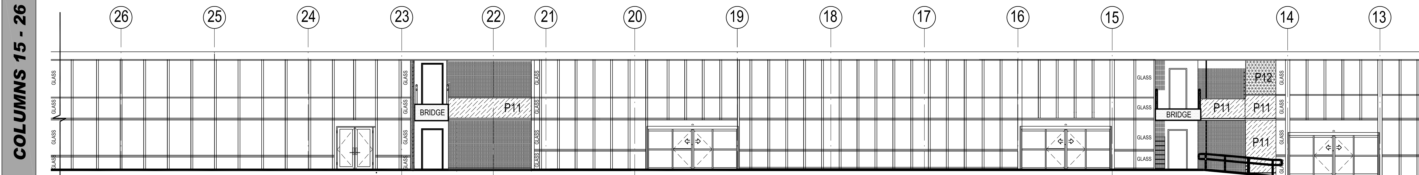
PERIMETER WALKWAY (OUTSIDE TICKETING B) CURTAIN WALL ELEVATIONS, SCALE: 1/8" = 1'-0"
