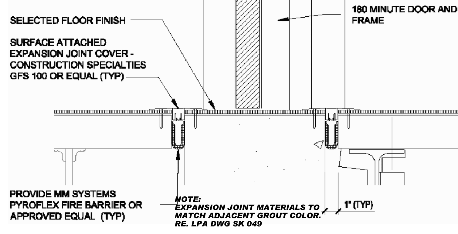
TYPICAL, ALL DRAWINGS! DETAIL: EXPANSION JOINT, SCALE: N.T.S.
