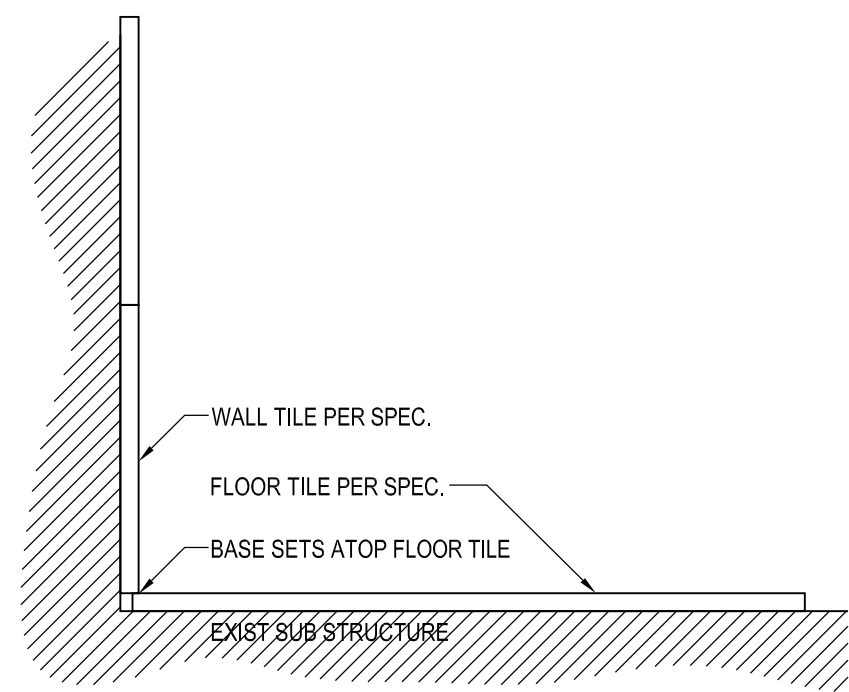
TYPICAL, ALL DRAWINGS! DETAIL: TILE WALL/TILE FLOOR, SCALE: N.T.S.
