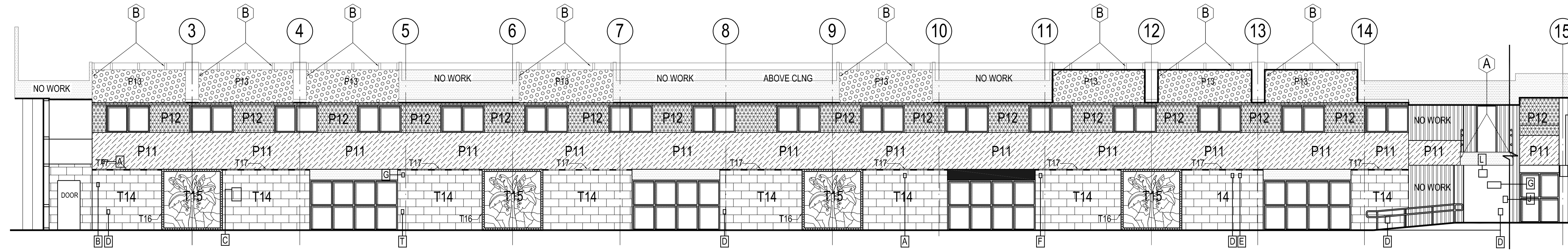
PERIMETER WALKWAY (OUTSIDE GATES 9-12) INTERIOR WALL ELEVATIONS, SCALE: 1/8" = 1'-0"
