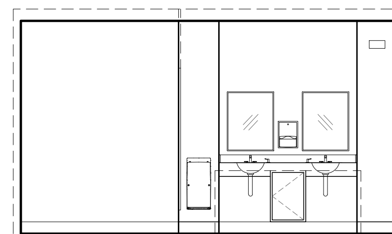
5 SECOND FLOOR WEST MENS RESTROOM SCALE: 1/4" = 1'-0"
