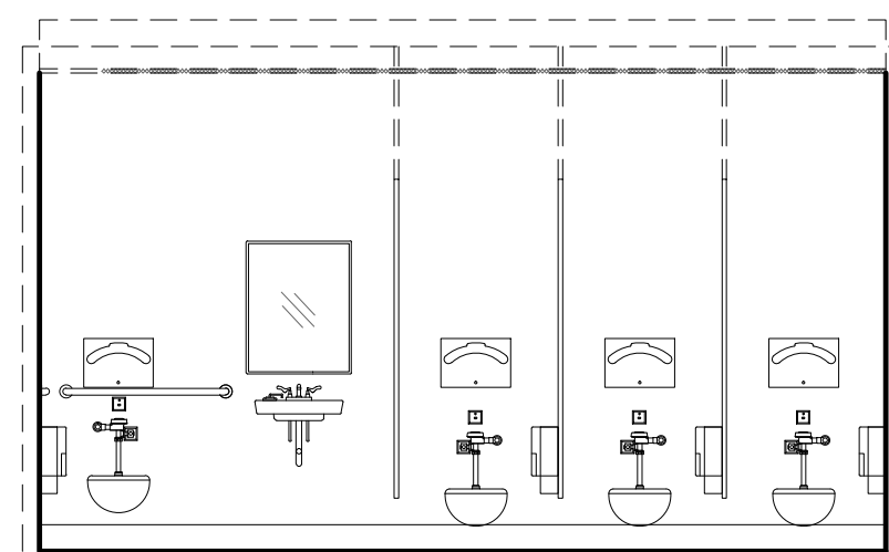
6 SECOND FLOOR WEST WOMENS RESTROOM SCALE: 1/4" = 1'-0"
