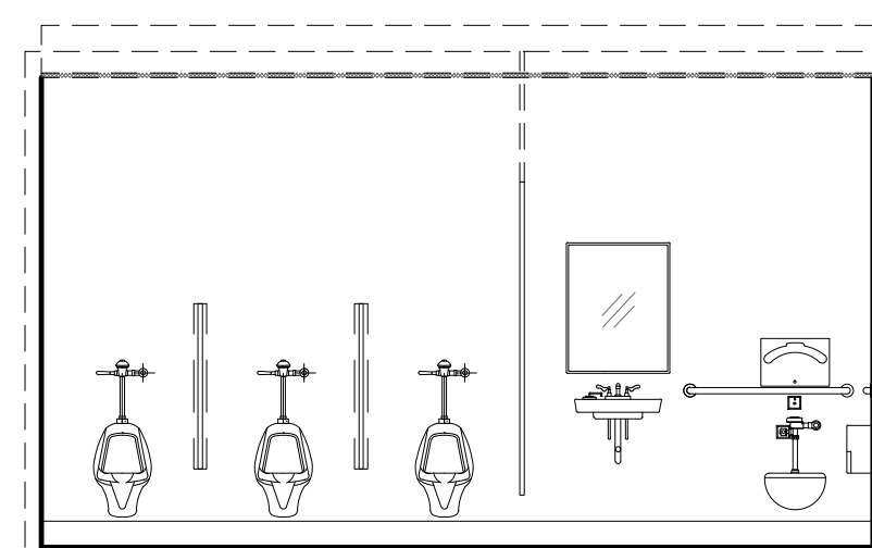
4 SECOND FLOOR WEST MENS RESTROOM SCALE: 1/4" = 1'-0"
