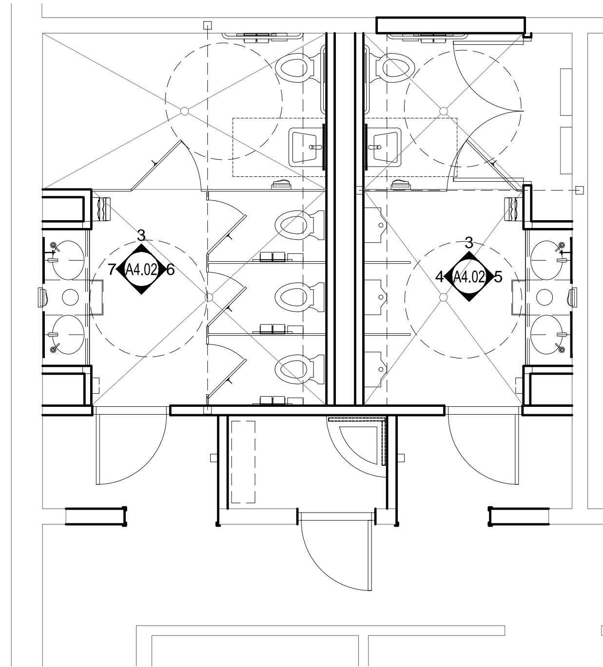
2 SECOND FLOOR NEW WORK PLAN ENLARGED WEST RESTROOM SCALE: 1/4" = 1'-0"
