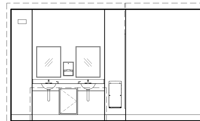
7 SECOND FLOOR WEST WOMENS RESTROOM SCALE: 1/4" = 1'-0"
