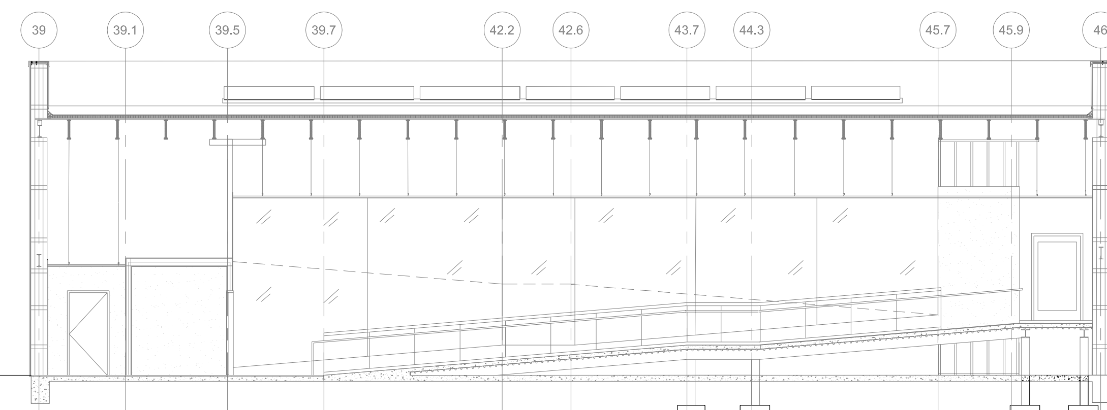
2 CROSSSECTION GATES 2-6 RAMP SCALE: 1/8" = 1'-0"
