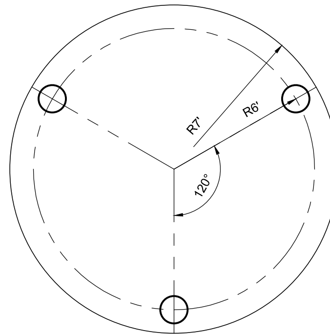
COLUMN / TRUNK LAYOUT 1/4" = 1'-0"
